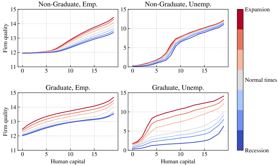
Figure 5: Search Policies
